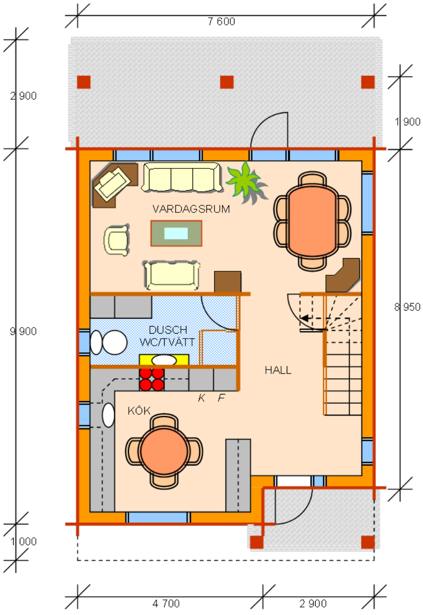
Bottenplan
