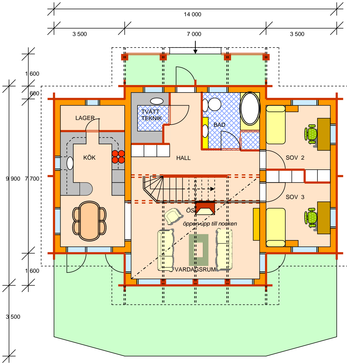
BOTTENPLAN
