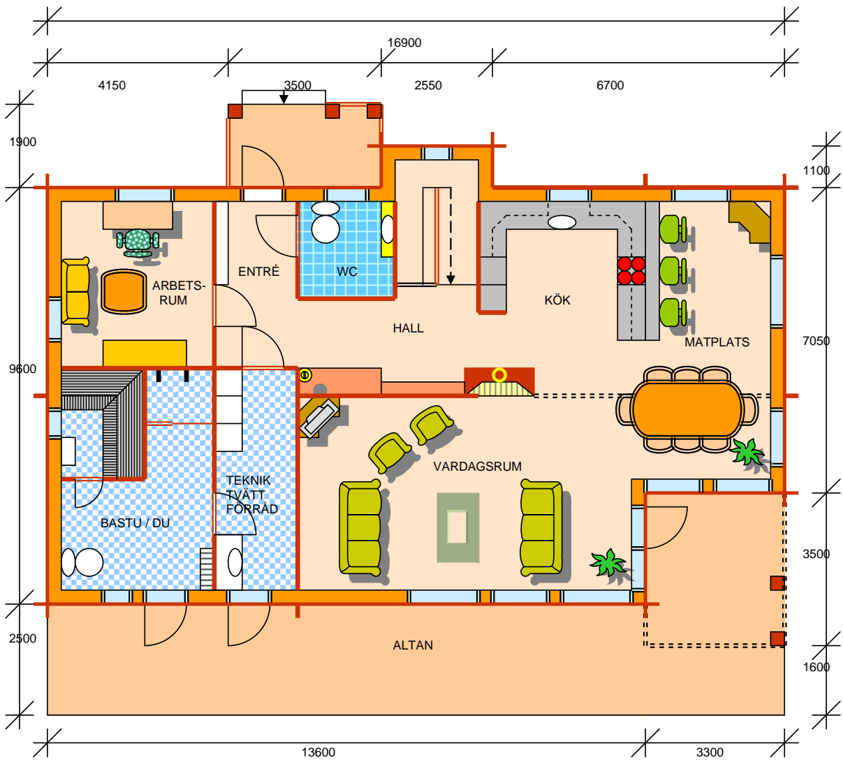
Bottenplan
